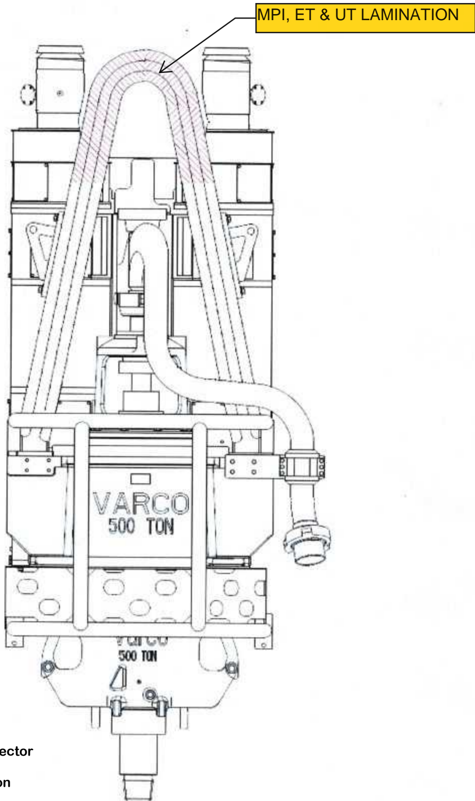
Figure 3: Integrated Swivel Bail
